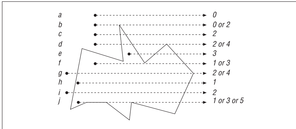
Figure 10-11. Is the point in the polygon? Count the edge crossings
